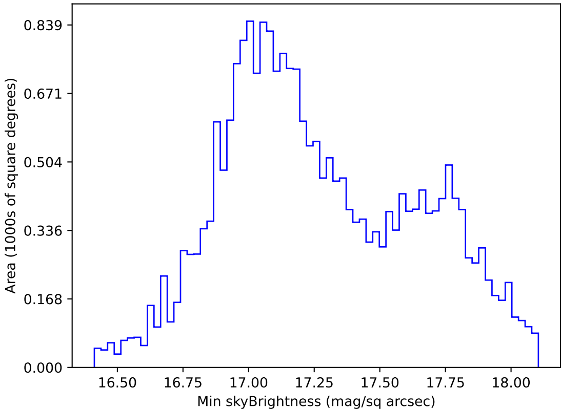
noroll_mjdp365_v3.4_10yrs All sky y band: Min skyBrightness
