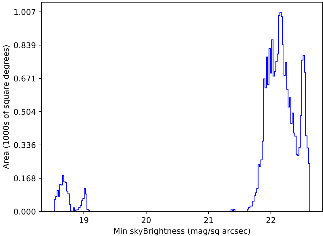
noroll_mjdp365_v3.4_10yrs All sky u band: Min skyBrightness
