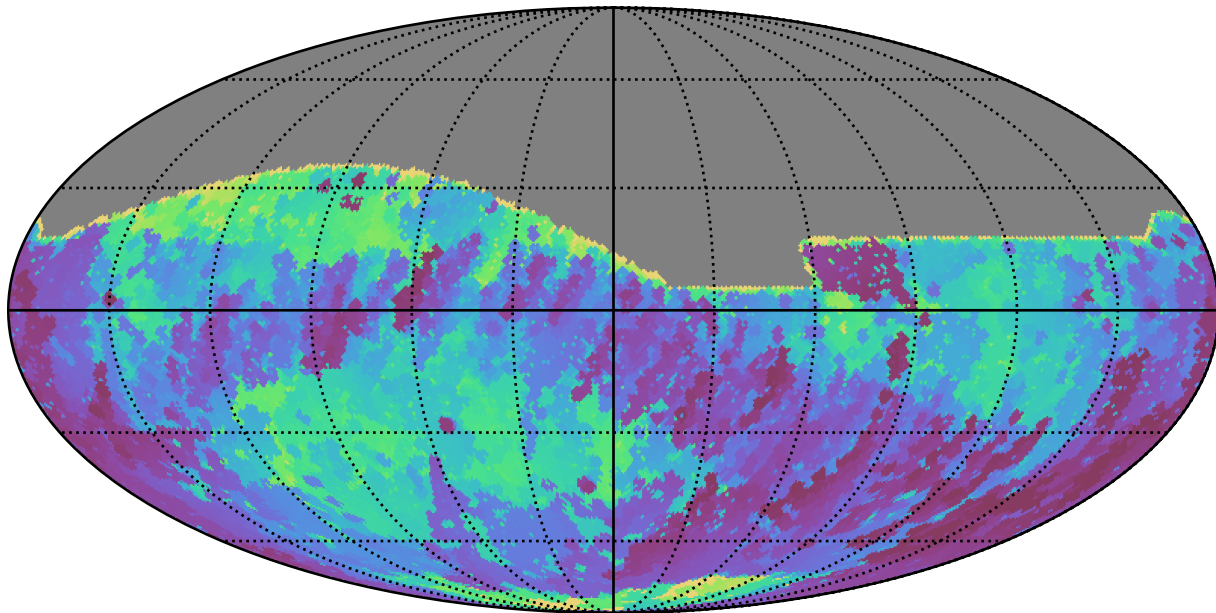
noroll_mjdp365_v3.4_10yrs All sky r band: Min skyBrightness
