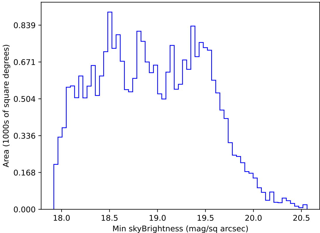
noroll_mjdp365_v3.4_10yrs All sky r band: Min skyBrightness
