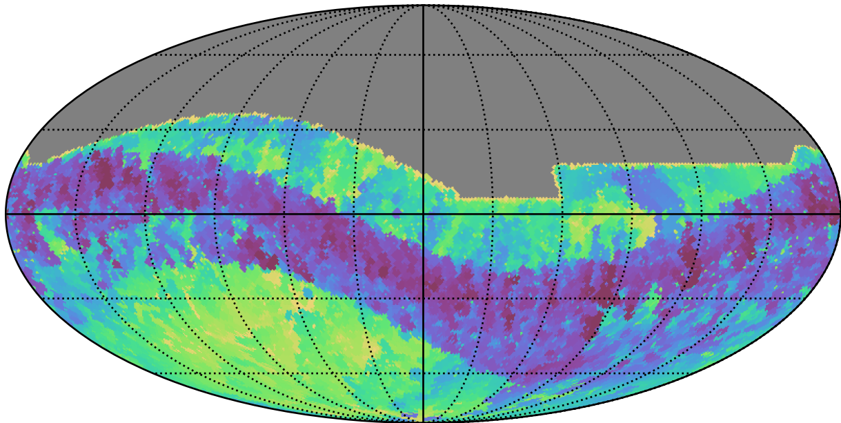
noroll_mjdp365_v3.4_10yrs All sky i band: Min skyBrightness
