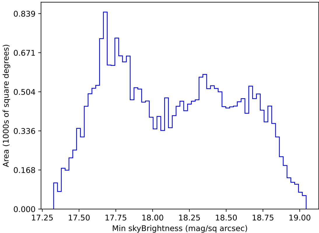
noroll_mjdp365_v3.4_10yrs All sky i band: Min skyBrightness
