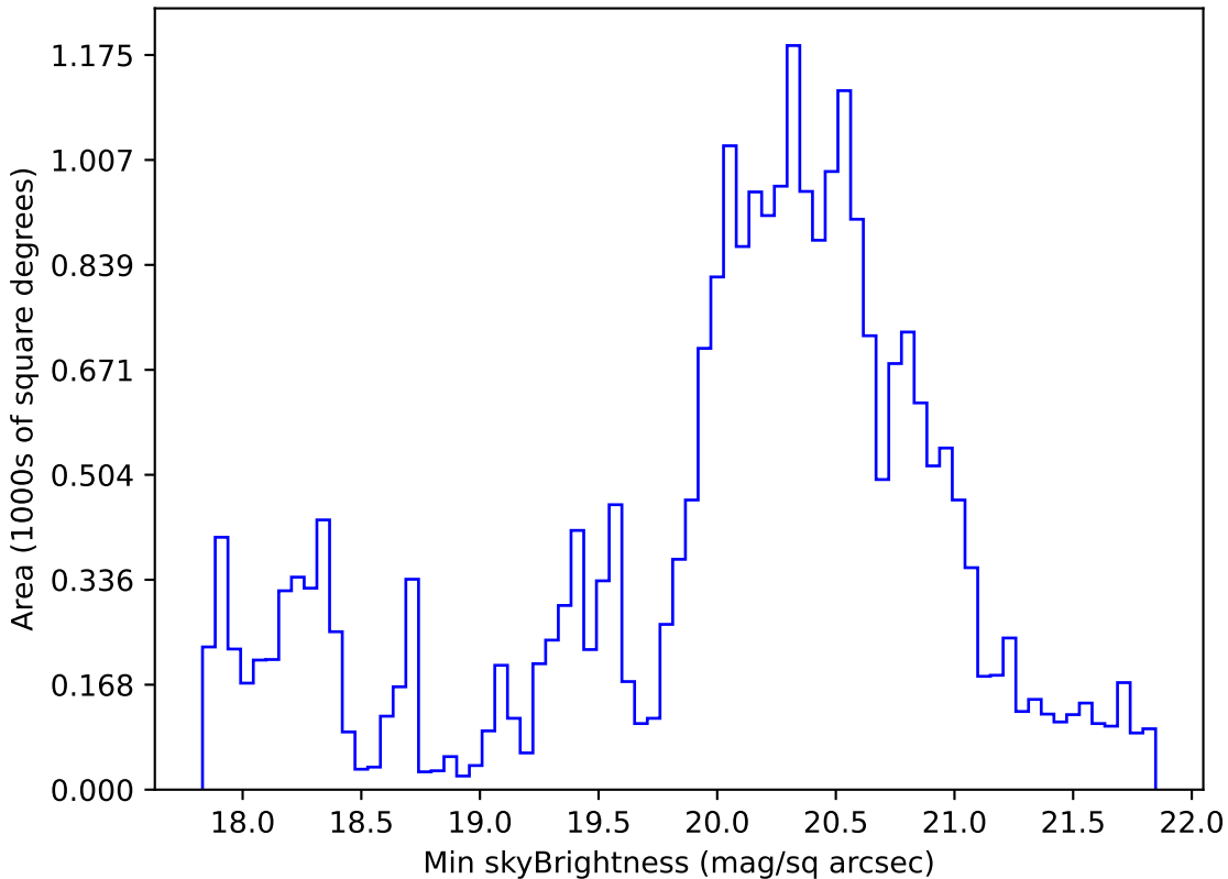
noroll_mjdp365_v3.4_10yrs All sky g band: Min skyBrightness
