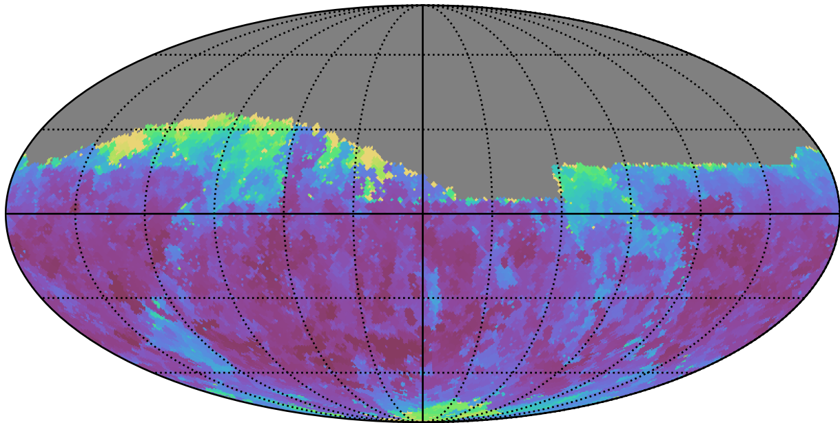
noroll_mjdp365_v3.4_10yrs Yr 1 z band: Min seeingGeom
