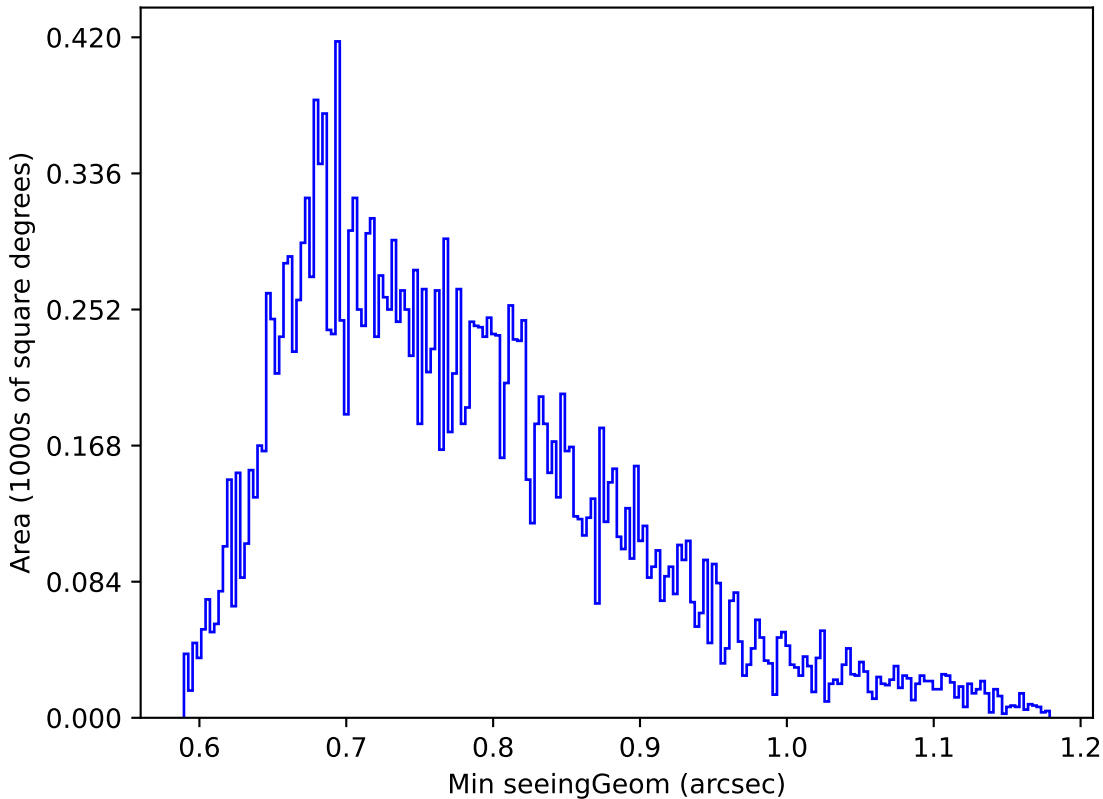
noroll_mjdp365_v3.4_10yrs Yr 1 u band: Min seeingGeom
