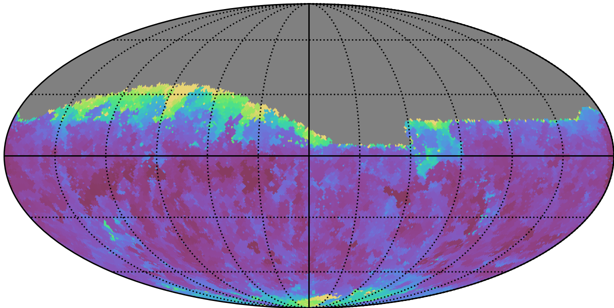
noroll_mjdp365_v3.4_10yrs Yr 1 r band: Min seeingGeom
