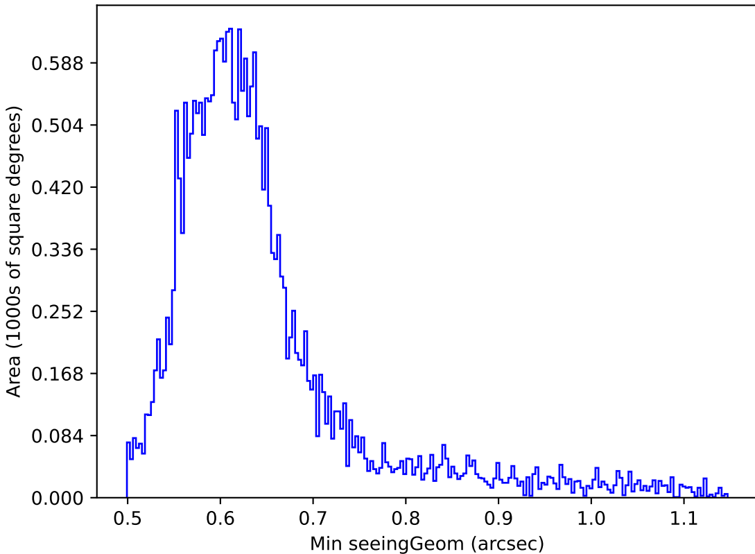
noroll_mjdp365_v3.4_10yrs Yr 1 r band: Min seeingGeom
