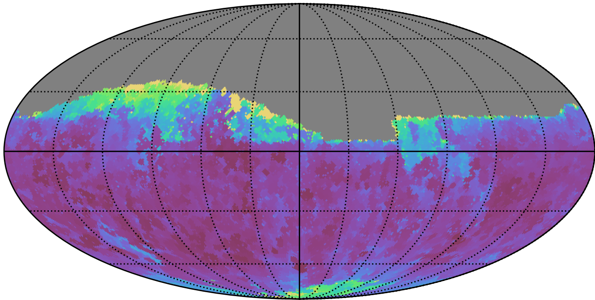
noroll_mjdp365_v3.4_10yrs Yr 1 i band: Min seeingGeom
