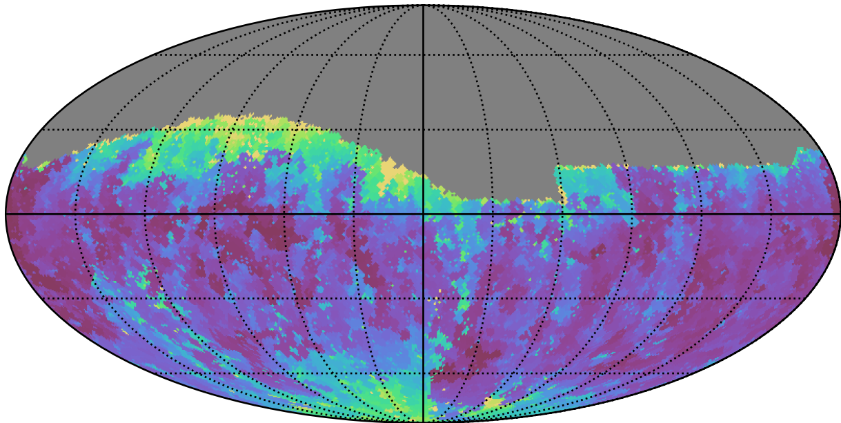
noroll_mjdp365_v3.4_10yrs Yr 1 g band: Min seeingGeom
