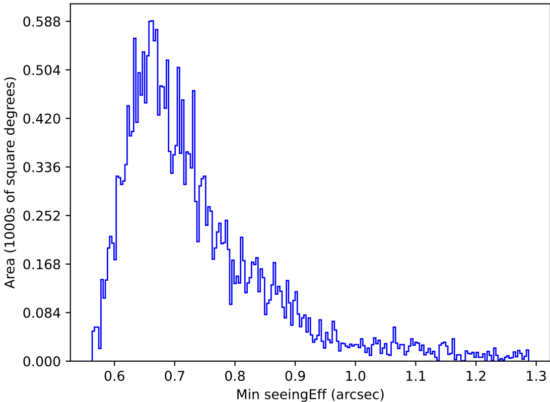
noroll_mjdp365_v3.4_10yrs Yr 1 z band: Min seeingEff
