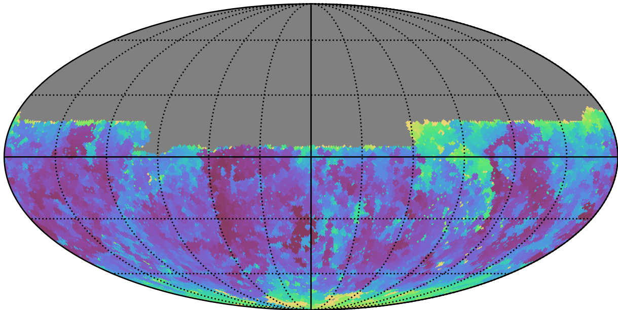
noroll_mjdp365_v3.4_10yrs Yr 1 y band: Min seeingEff
