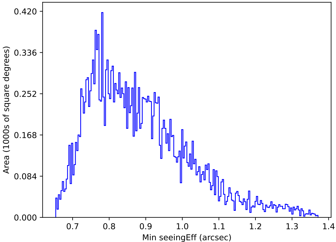
noroll_mjdp365_v3.4_10yrs Yr 1 u band: Min seeingEff
