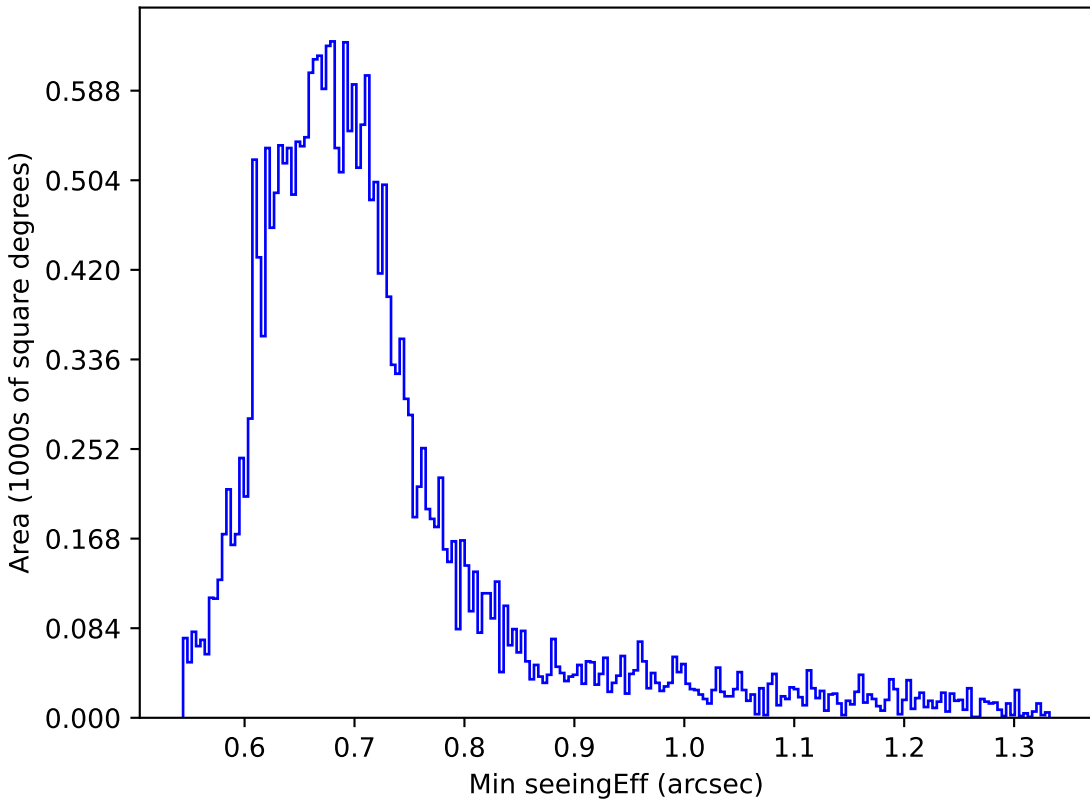
noroll_mjdp365_v3.4_10yrs Yr 1 r band: Min seeingEff
