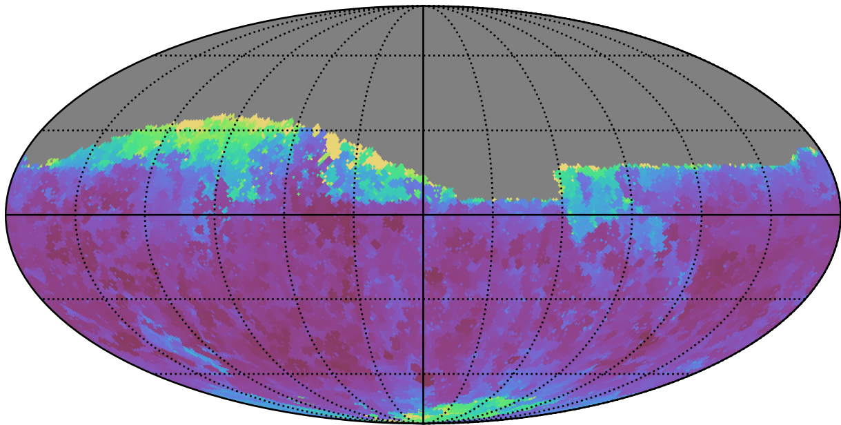
noroll_mjdp365_v3.4_10yrs Yr 1 i band: Min seeingEff
