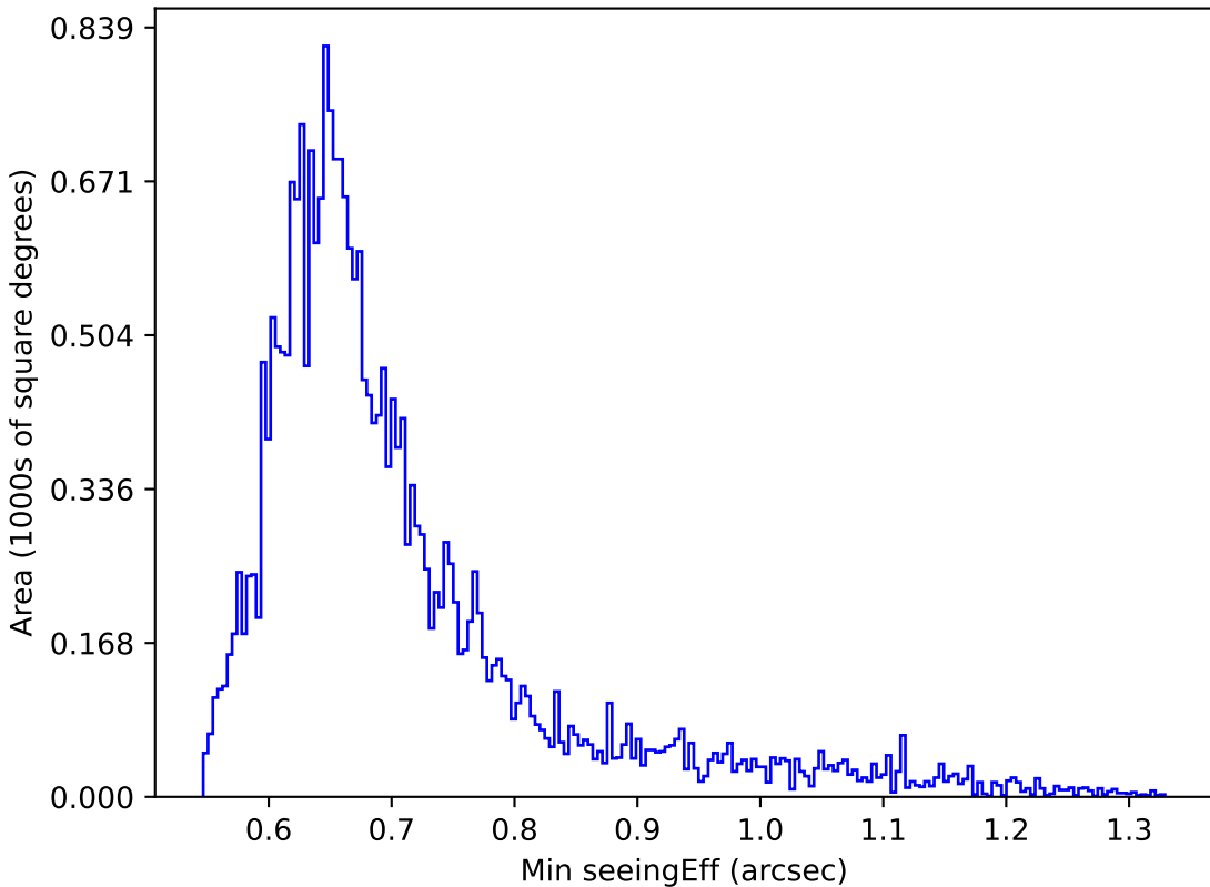
noroll_mjdp365_v3.4_10yrs Yr 1 i band: Min seeingEff
