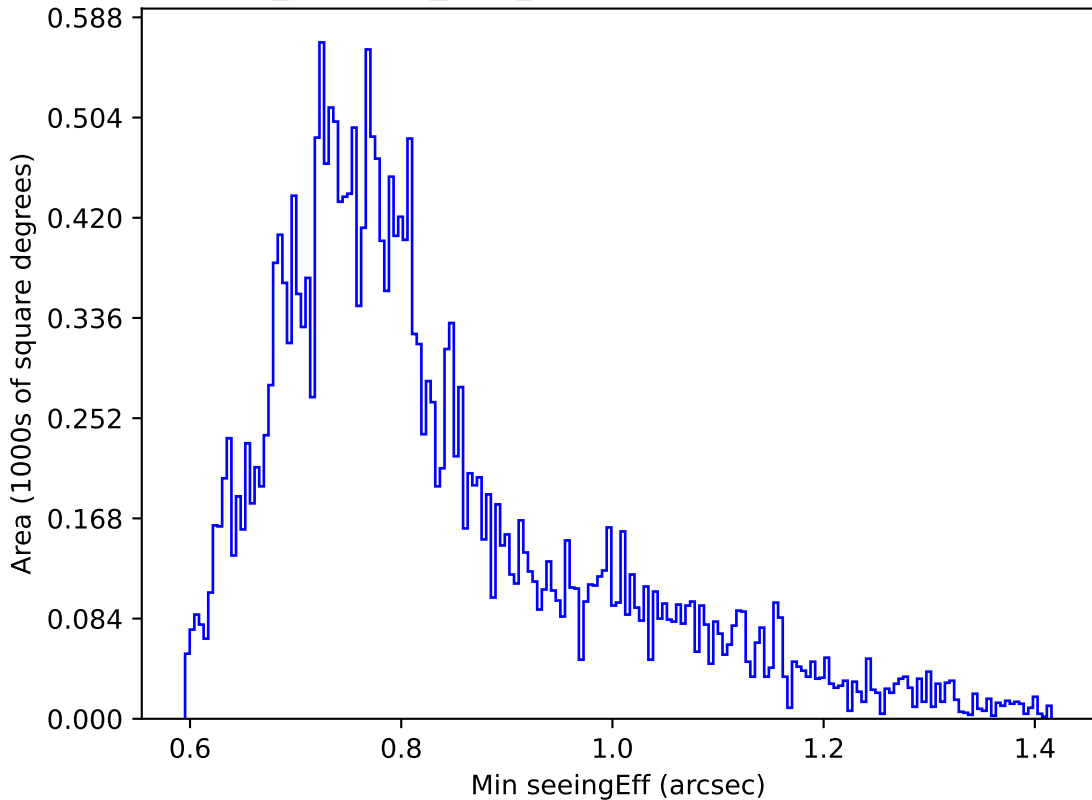
noroll_mjdp365_v3.4_10yrs Yr 1 g band: Min seeingEff
