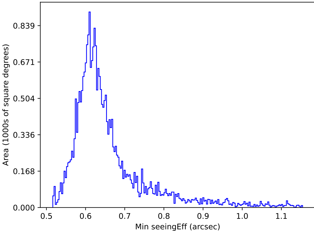
noroll_mjdp365_v3.4_10yrs Yr 1 all bands: Min seeingEff
