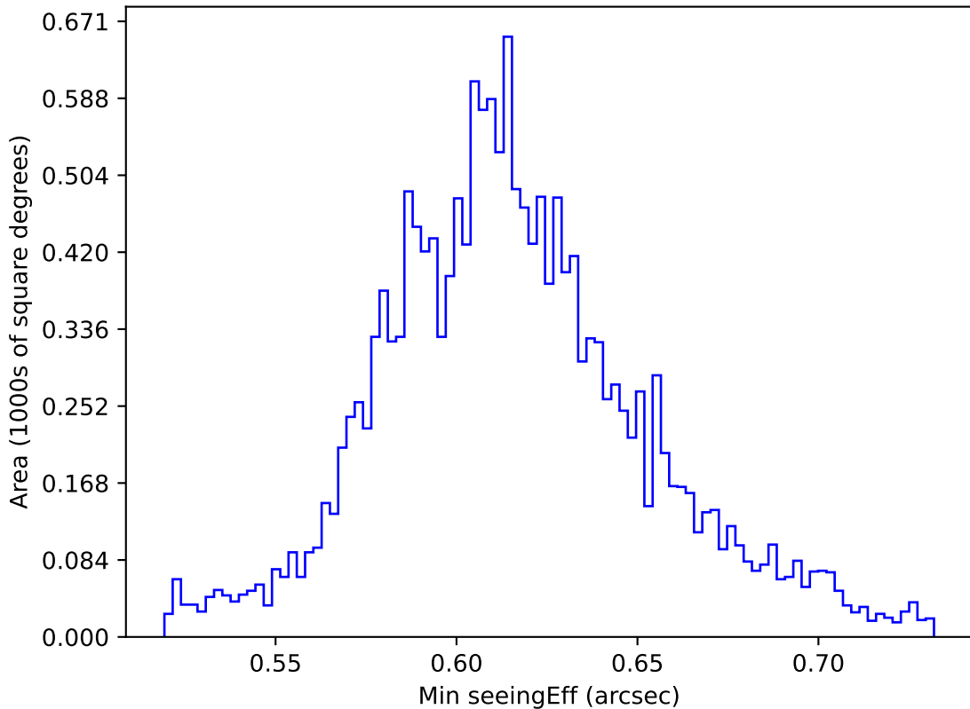
noroll_mjdp365_v3.4_10yrs WFD z band: Min seeingEff
