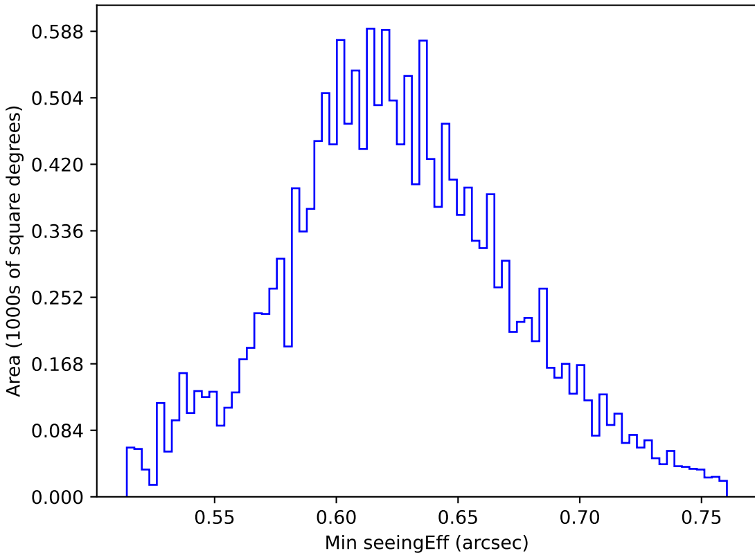
noroll_mjdp365_v3.4_10yrs WFD y band: Min seeingEff
