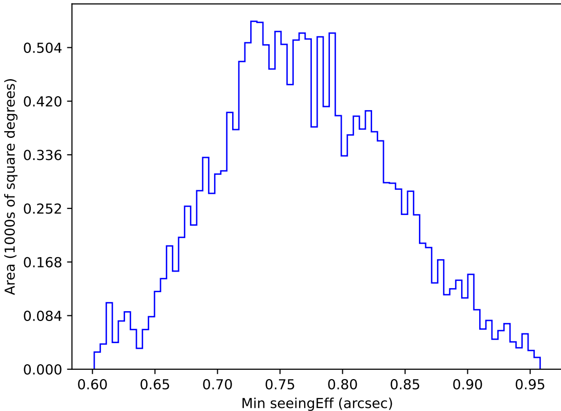
noroll_mjdp365_v3.4_10yrs WFD u band: Min seeingEff
