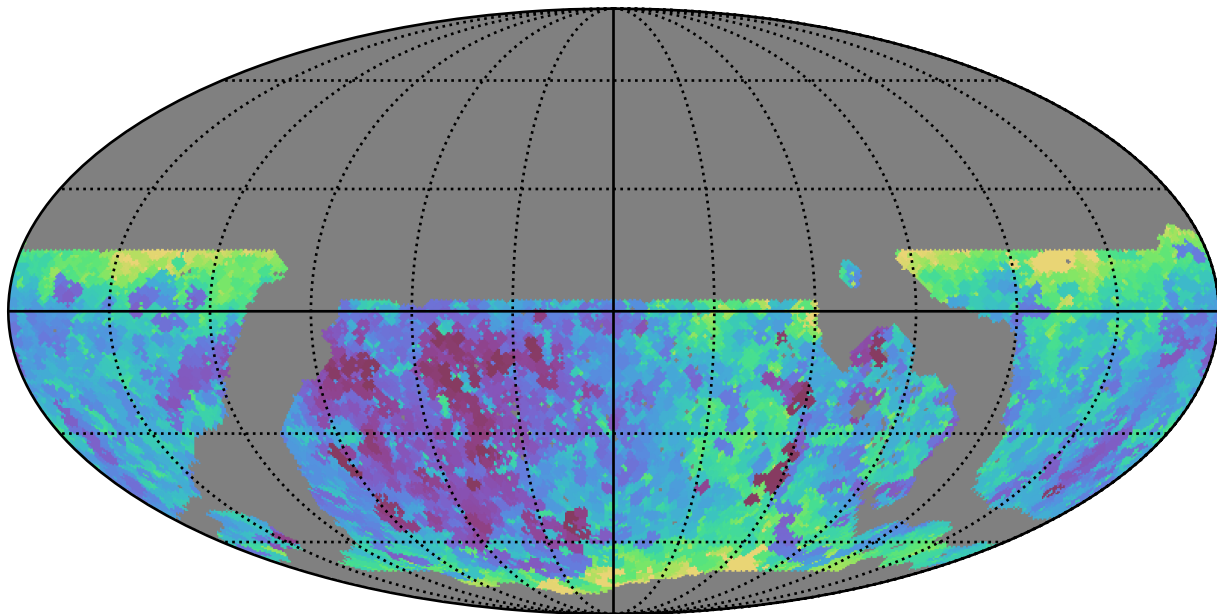
noroll_mjdp365_v3.4_10yrs WFD r band: Min seeingEff
