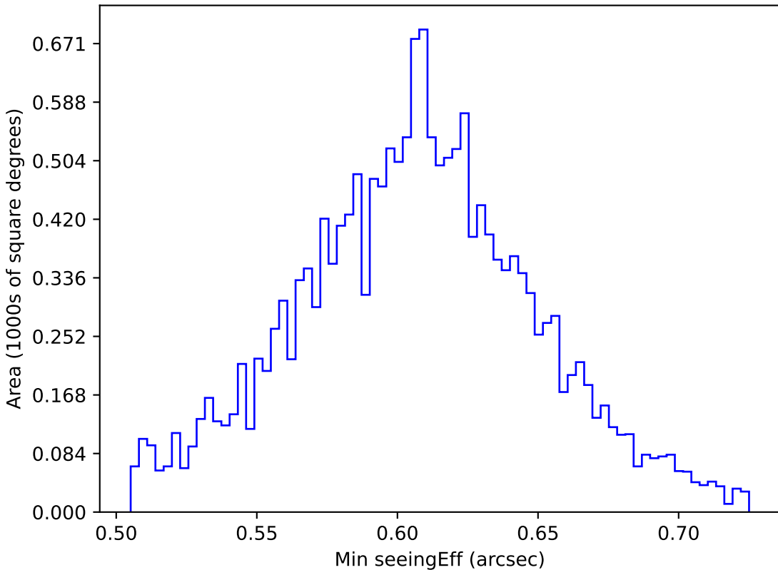
noroll_mjdp365_v3.4_10yrs WFD r band: Min seeingEff
