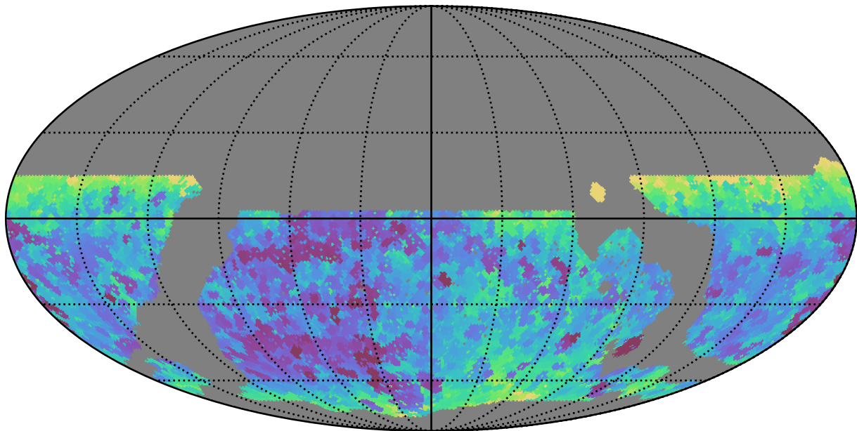
noroll_mjdp365_v3.4_10yrs WFD i band: Min seeingEff
