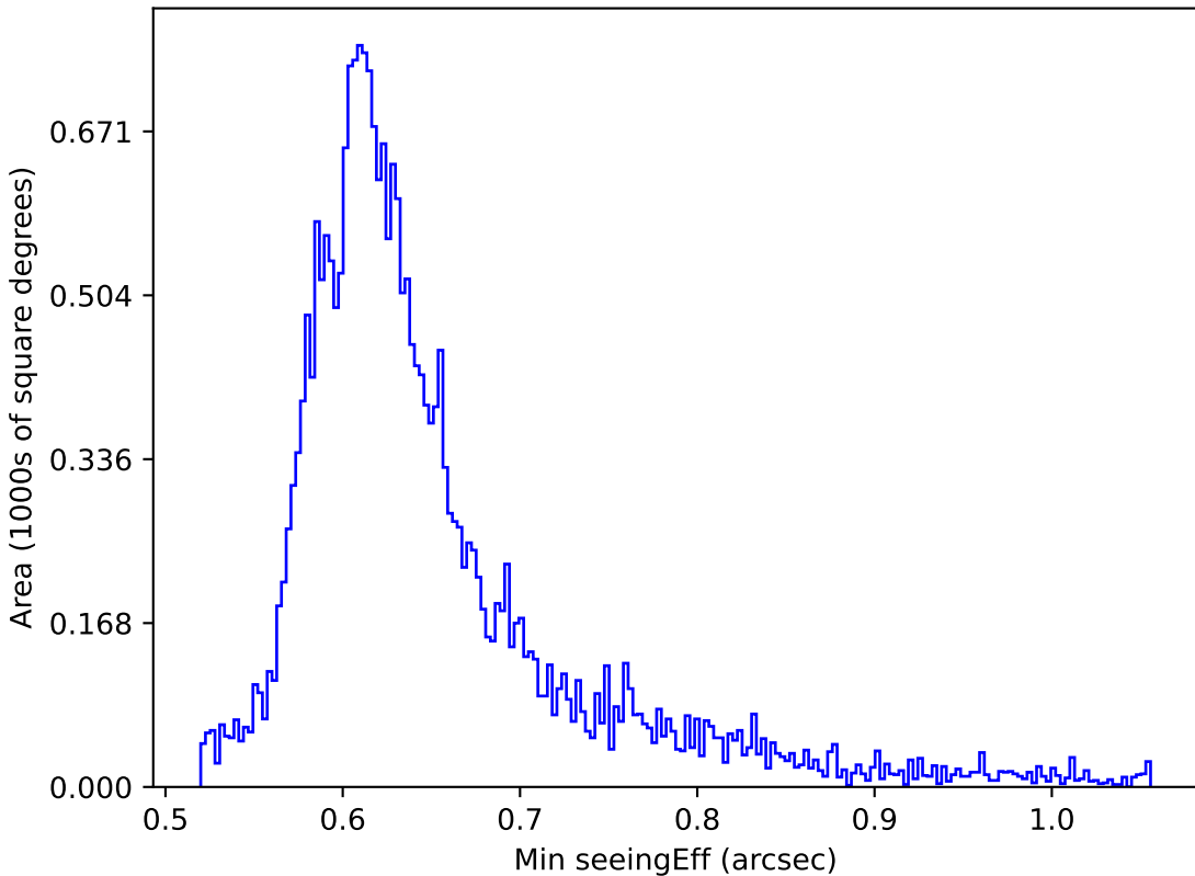
noroll_mjdp365_v3.4_10yrs All sky z band: Min seeingEff
