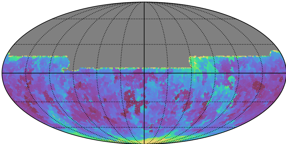
noroll_mjdp365_v3.4_10yrs All sky u band: Min seeingEff
