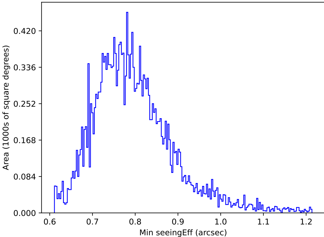
noroll_mjdp365_v3.4_10yrs All sky u band: Min seeingEff
