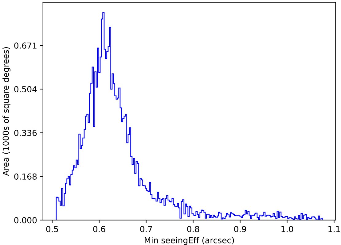
noroll_mjdp365_v3.4_10yrs All sky r band: Min seeingEff
