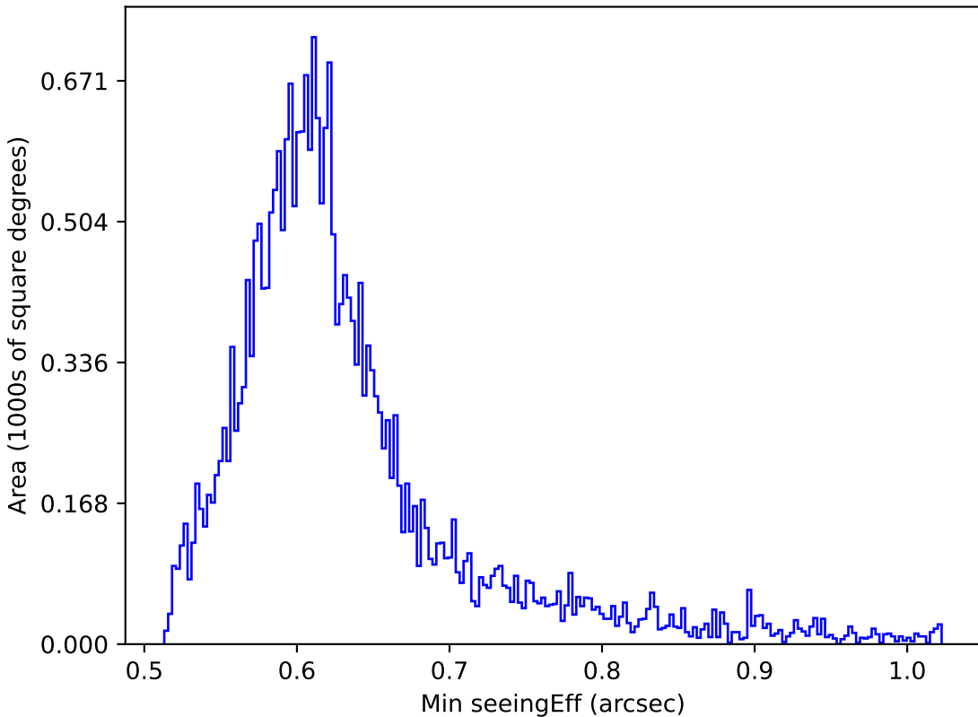
noroll_mjdp365_v3.4_10yrs All sky i band: Min seeingEff
