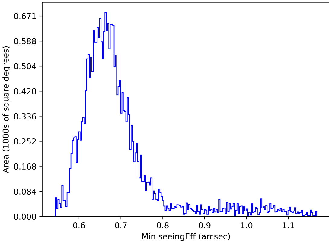
noroll_mjdp365_v3.4_10yrs All sky g band: Min seeingEff
