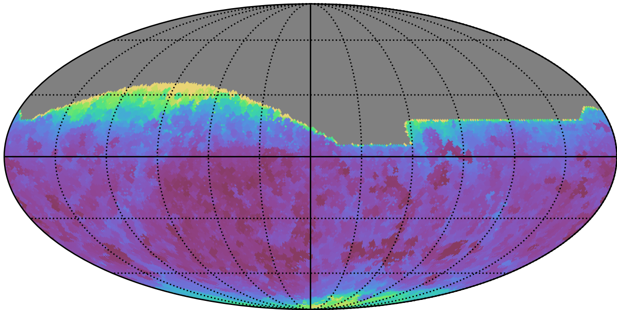
noroll_mjdp365_v3.4_10yrs All sky all bands: Min seeingEff
