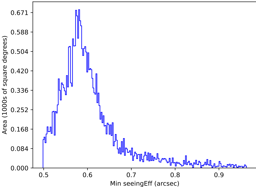
noroll_mjdp365_v3.4_10yrs All sky all bands: Min seeingEff
