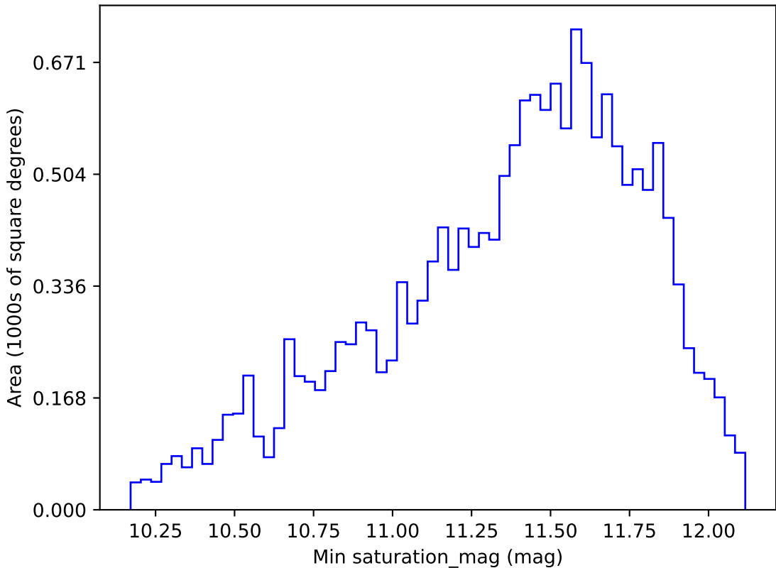
noroll_mjdp365_v3.4_10yrs WFD y band: Min saturation_mag
