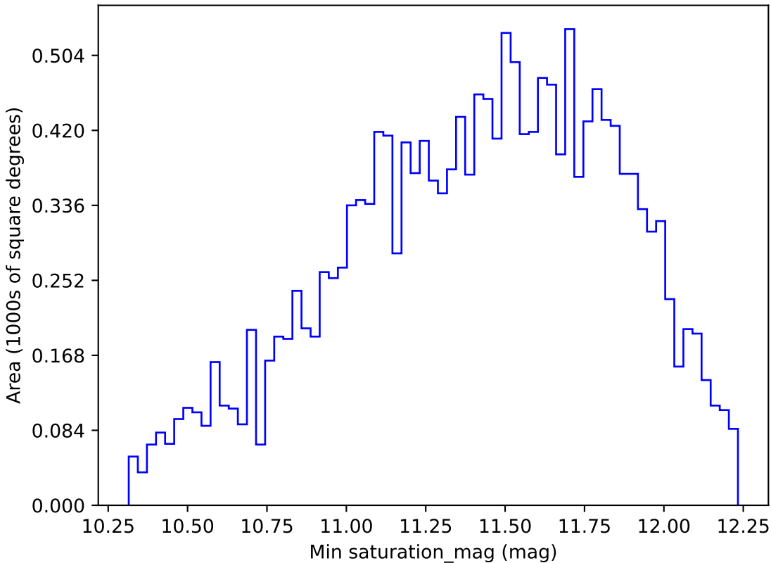
noroll_mjdp365_v3.4_10yrs WFD u band: Min saturation_mag
