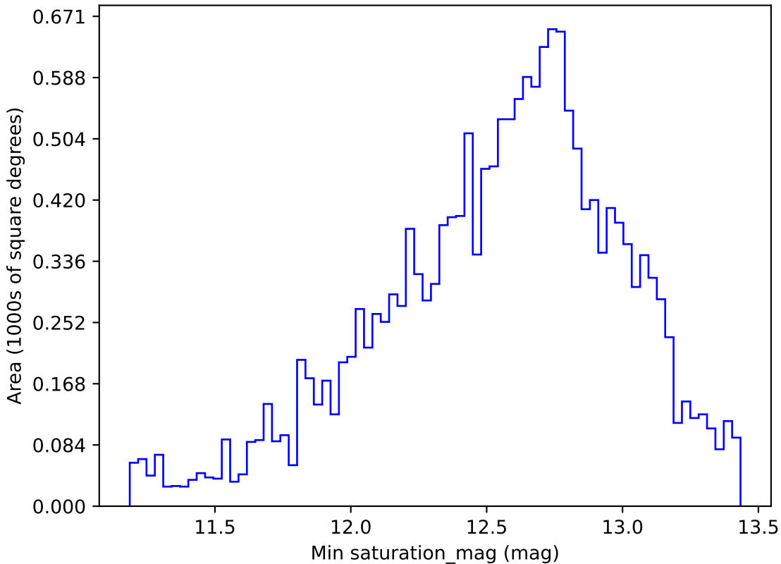
noroll_mjdp365_v3.4_10yrs WFD r band: Min saturation_mag
