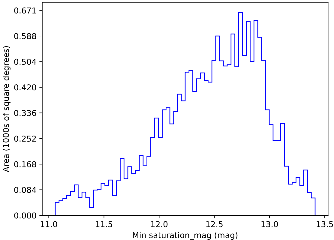
noroll_mjdp365_v3.4_10yrs WFD i band: Min saturation_mag
