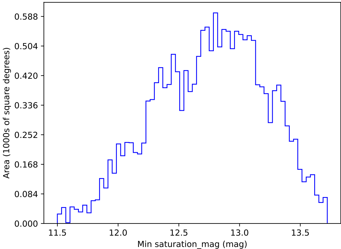
noroll_mjdp365_v3.4_10yrs WFD g band: Min saturation_mag
