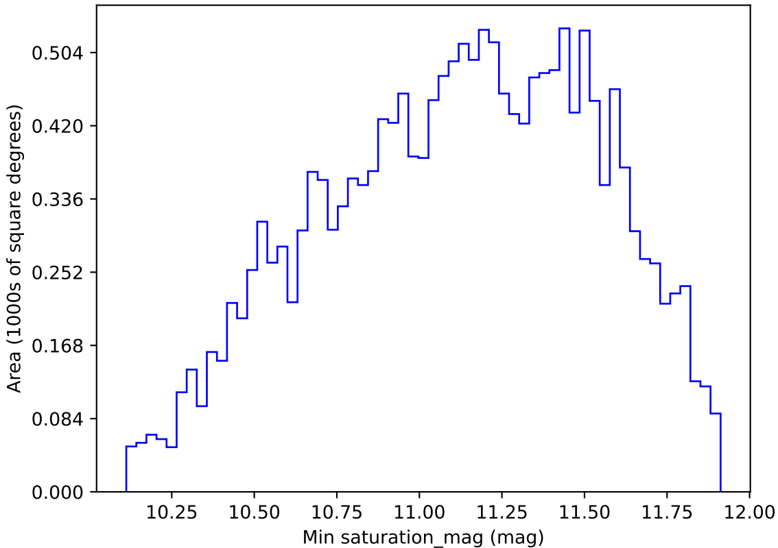
noroll_mjdp365_v3.4_10yrs WFD all bands: Min saturation_mag
