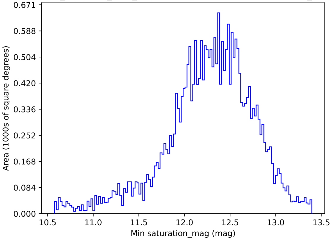
noroll_mjdp365_v3.4_10yrs All sky z band: Min saturation_mag
