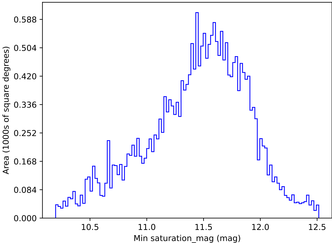
noroll_mjdp365_v3.4_10yrs All sky y band: Min saturation_mag
