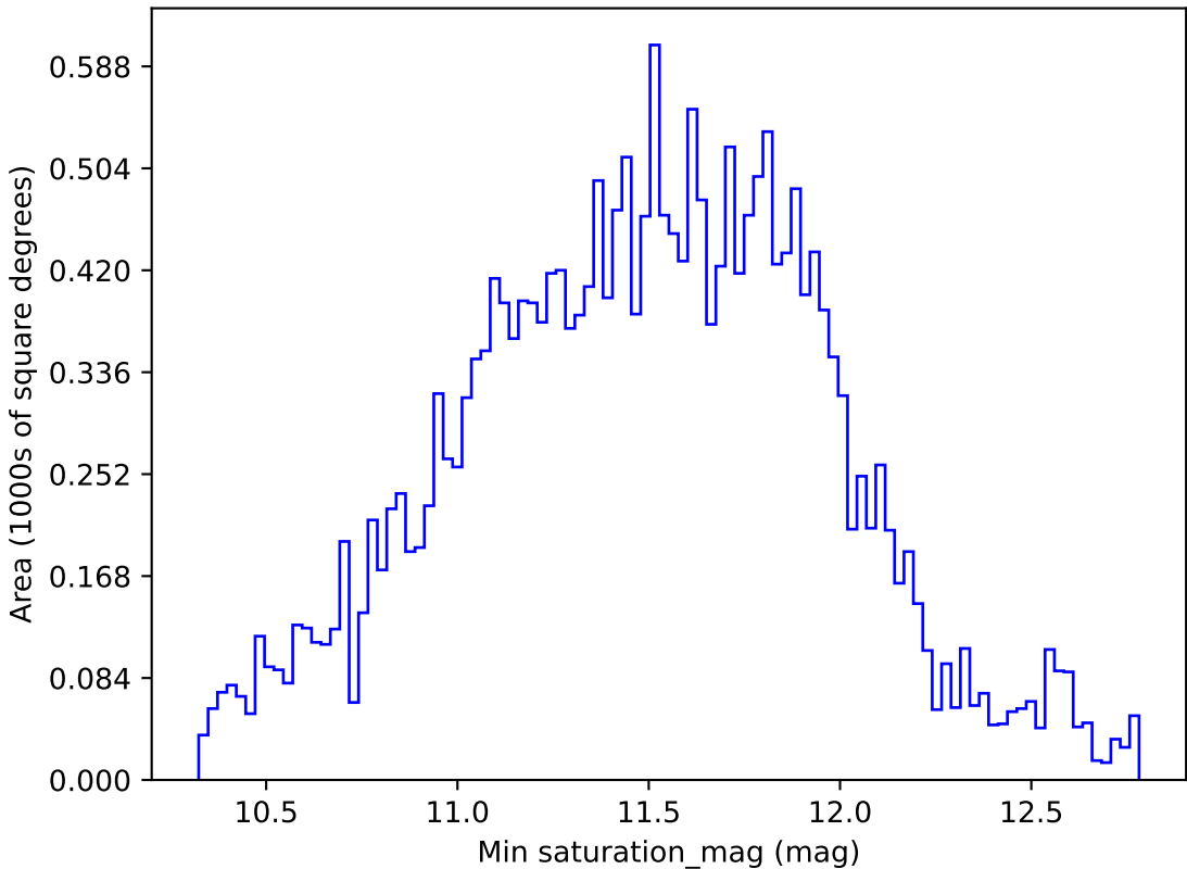
noroll_mjdp365_v3.4_10yrs All sky u band: Min saturation_mag
