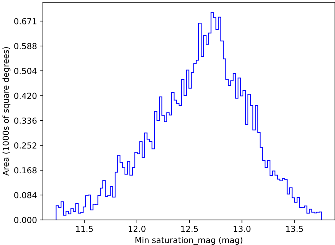
noroll_mjdp365_v3.4_10yrs All sky r band: Min saturation_mag
