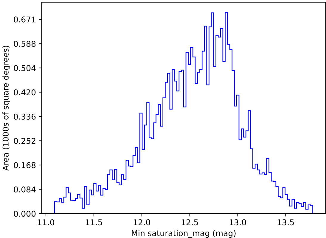
noroll_mjdp365_v3.4_10yrs All sky i band: Min saturation_mag
