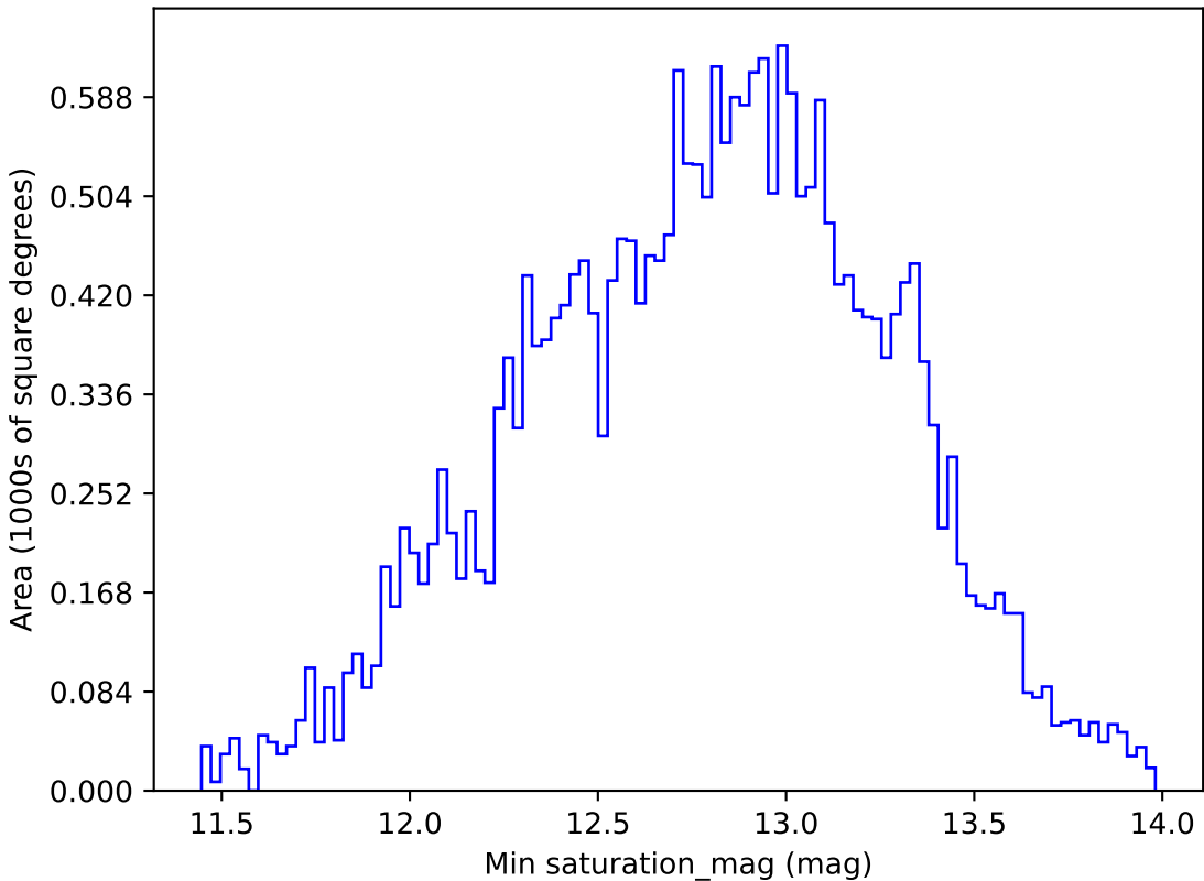
noroll_mjdp365_v3.4_10yrs All sky g band: Min saturation_mag
