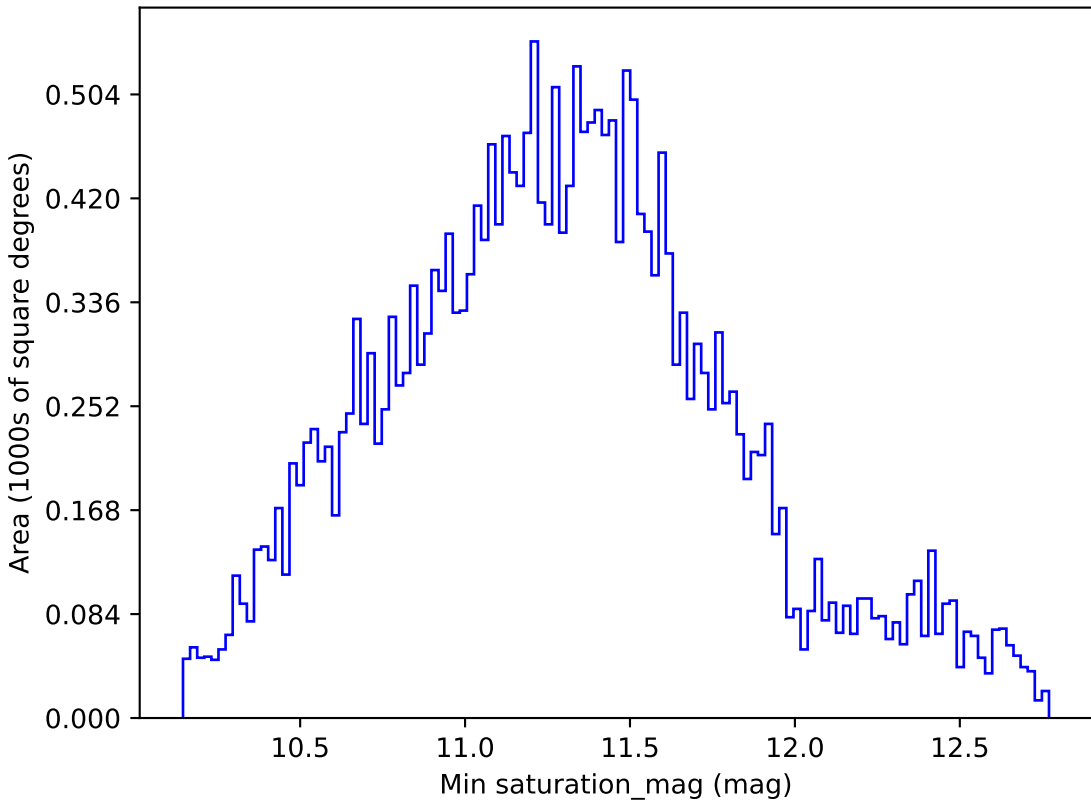
noroll_mjdp365_v3.4_10yrs All sky all bands: Min saturation_mag
