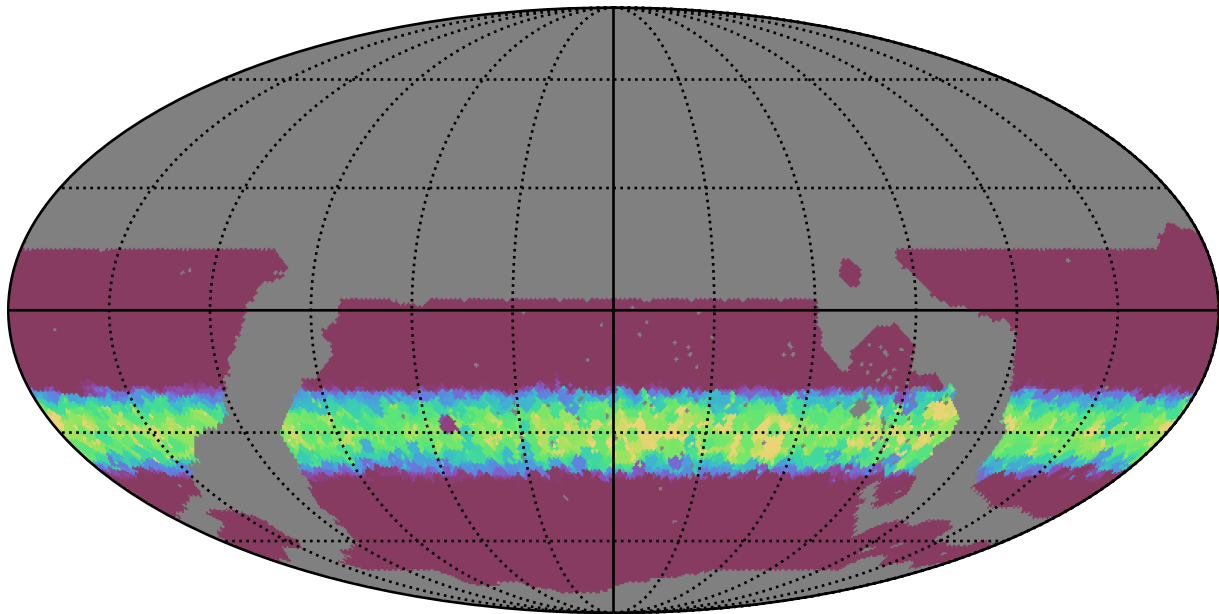
noroll_mjdp365_v3.4_10yrs WFD z band: Min normairmass
