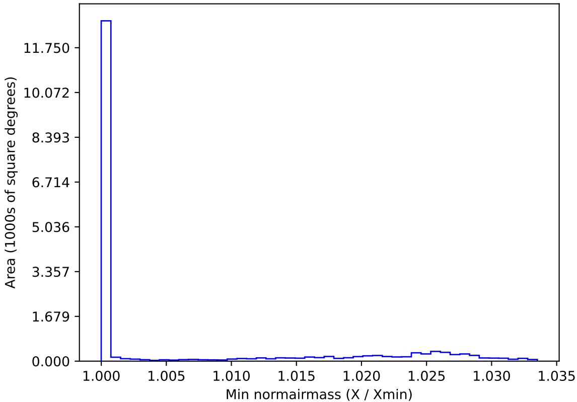
noroll_mjdp365_v3.4_10yrs WFD z band: Min normairmass
